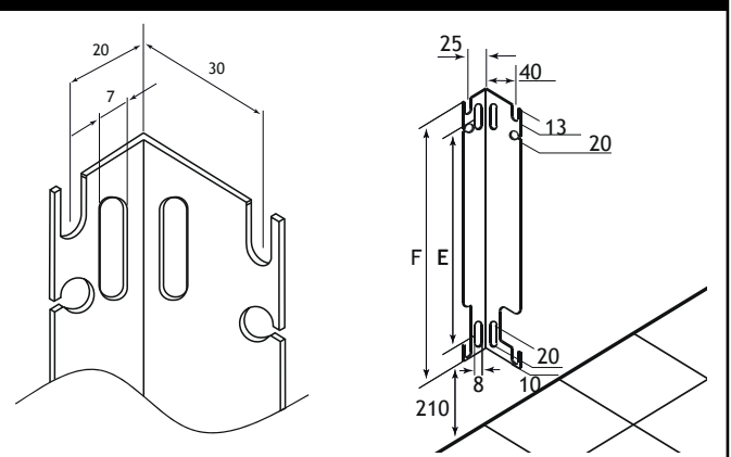
Wall Brackets
