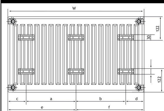
Bracket Positioning
